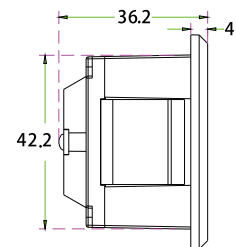
侧视图1 Side view 1
