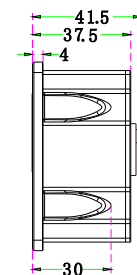
侧视图 Side view
