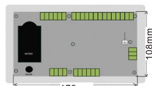
后视图 Rear view
